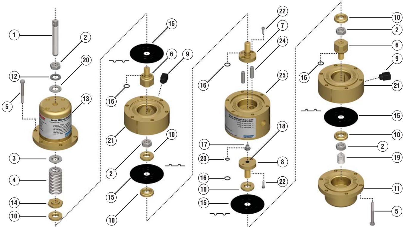
Figure 5 - DPS-2-200 Non-Bleed Sensor Exploded View
